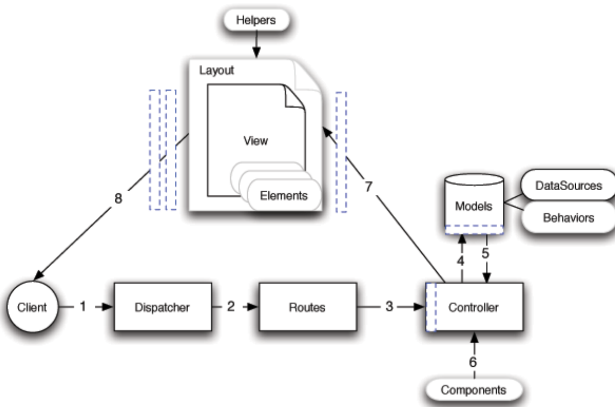
Figure 3.1: Flow diagram showing a typical CakePHP request
